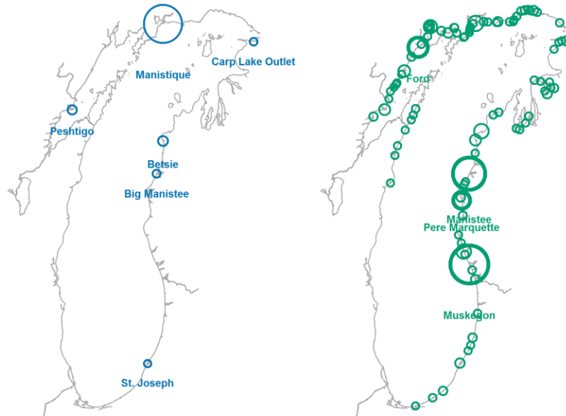
Figure 2. LEFT: Estimated index of adult sea lampreys during the spring spawning migration, 2015. Circle size corresponds to estimated number of adults from mark-recapture studies (blue) and model predictions (orange). All index streams are identified. RIGHT: Maximum estimated number of larval sea lampreys in each stream surveyed during 1995-2012. Tributaries composing over half of the lake-wide larval population estimate are identified (Muskegon 4,500,000; Manistee 3,600,000; Ford 1,800,000; Pere Marquette 1,400,000).
